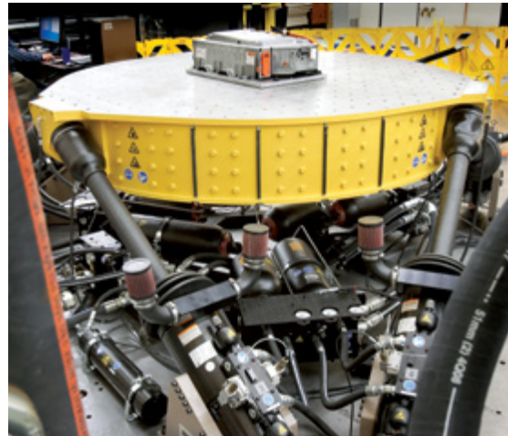
Model 353 Hexapod MAST System
