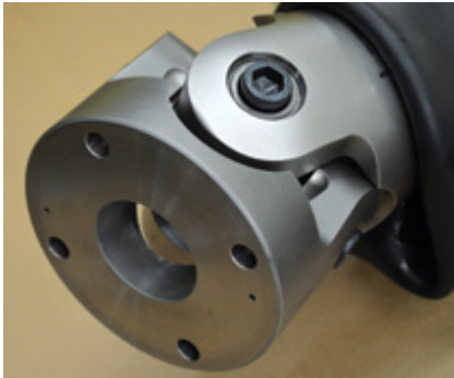
Durable, maintenance-free swivels feature low-friction zero-backlash bearings
