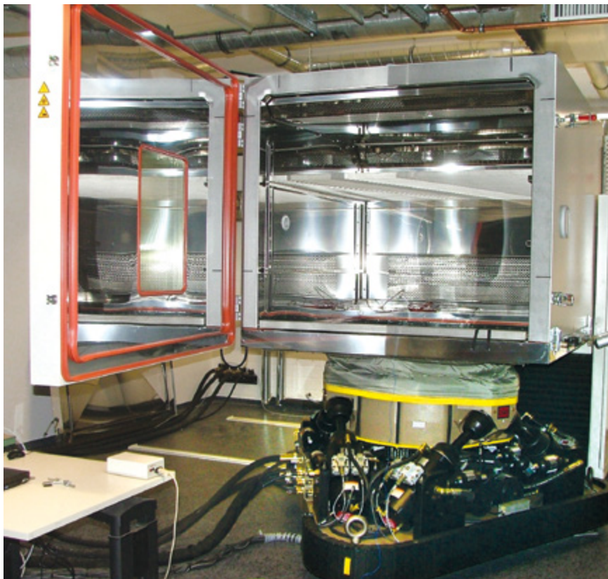
Model 353 MAST system with integrated environmental chamber at PLDS Automotive Test Laboratory in Wetzlar Germany (Photo courtesy of PLDS Germany GmbH)
